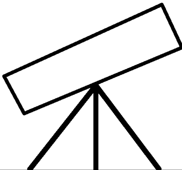
TELESCOPE VIEW
