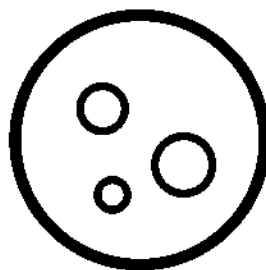
Ariel
