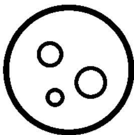
Miranda
