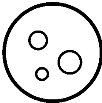
Miranda
